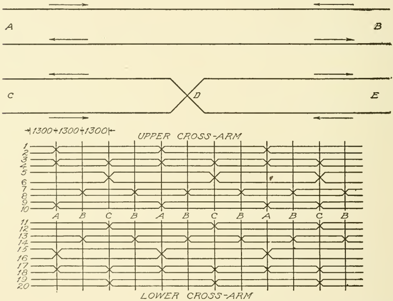
Fig. 22. Transposition Diagram of Ten Two-Wire Circuits to Reduce Mutual-Inductance
